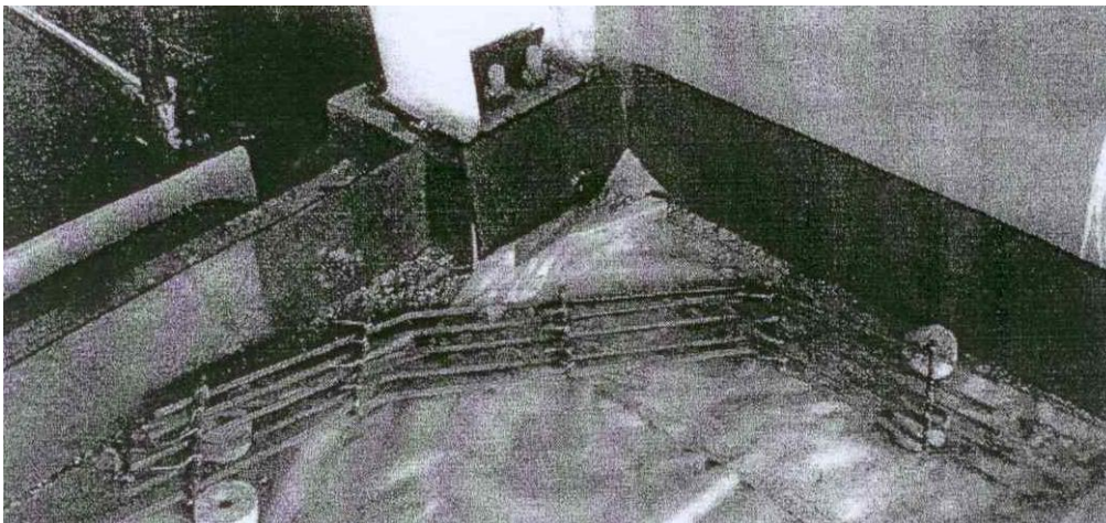
Column Isolation & Auxiliary Reinforcement at Column in Corners.
